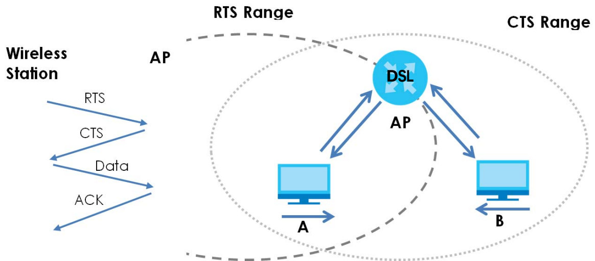
Figure 246 RTS/CTS
