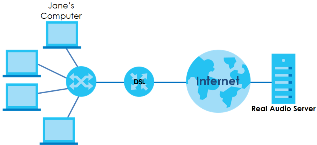
Figure 136 Trigger Port Forwarding Process: Example
