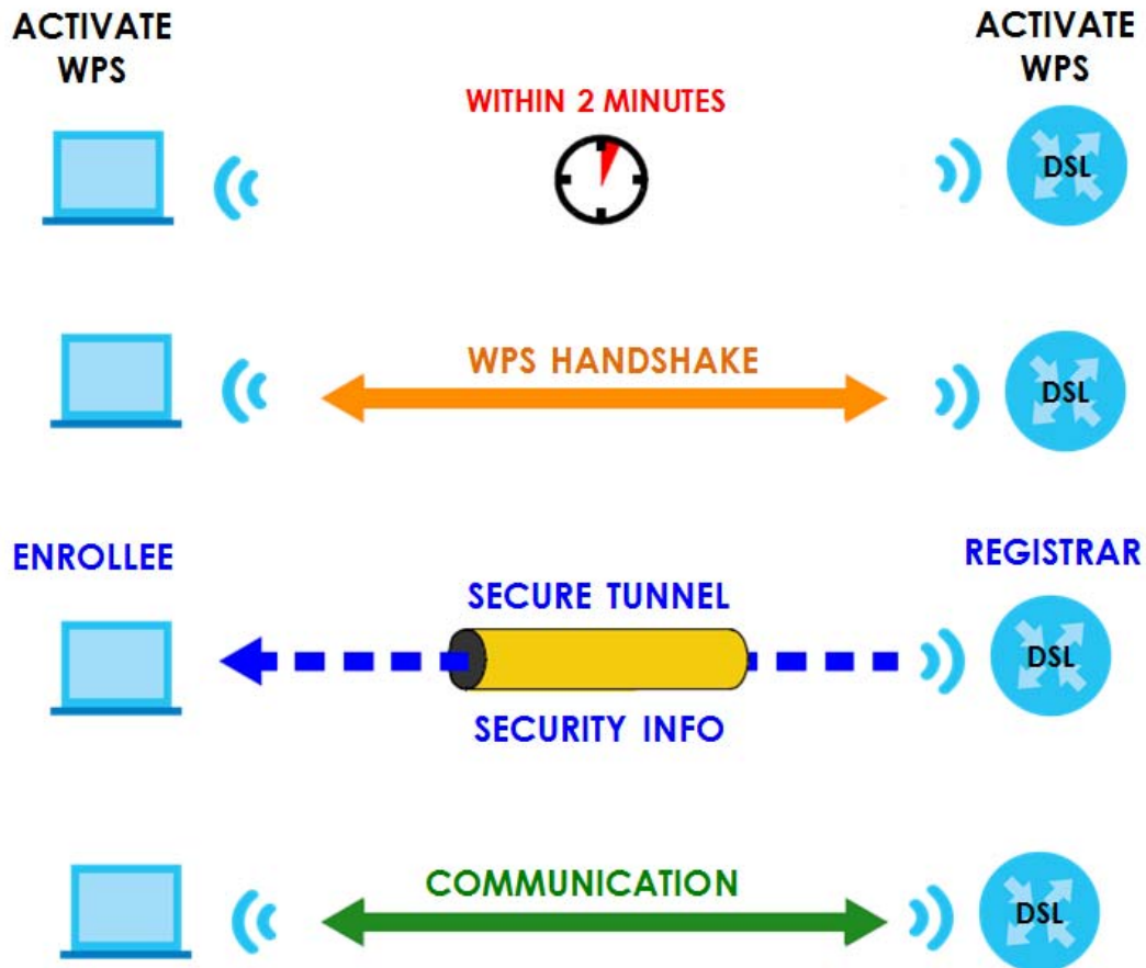
Figure 103 How WPS works
