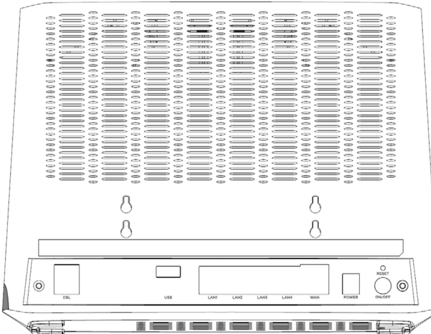
Figure 30 VMG3927-Bx0A Rear Panel
