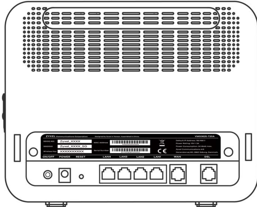
Figure 26 VMG3625-T20A Rear Panel
