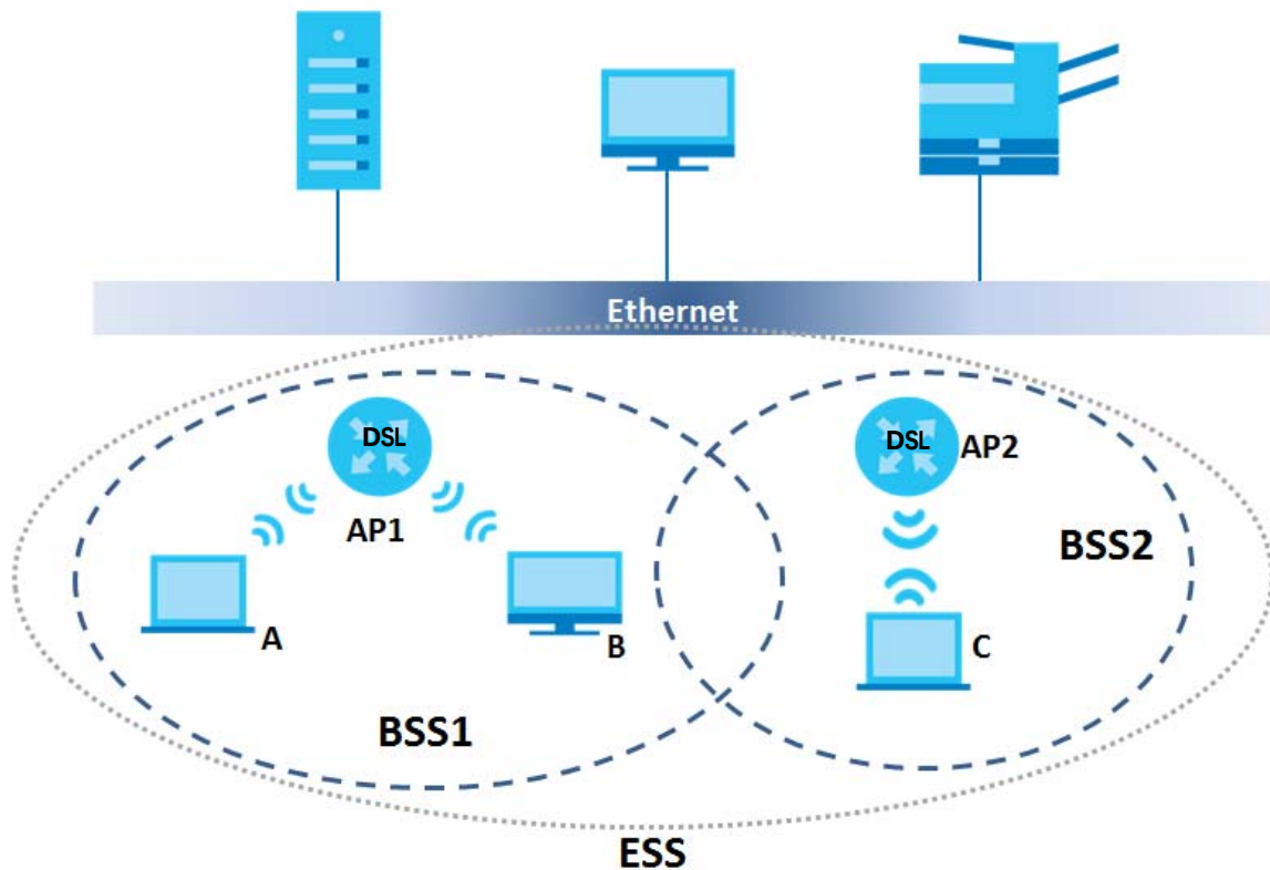
Figure 245 Infrastructure WLAN
