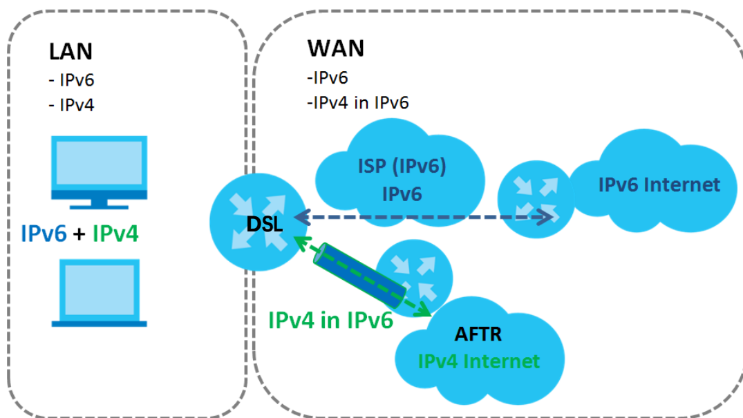
Figure 74 Dual Stack Lite
