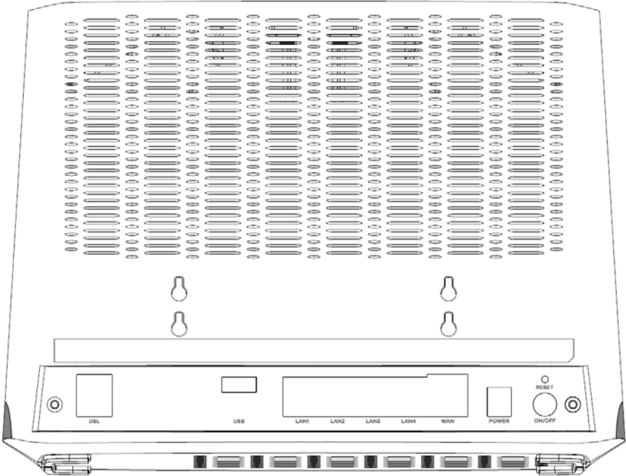
Figure 37 XMG3927-B50A Rear Panel
