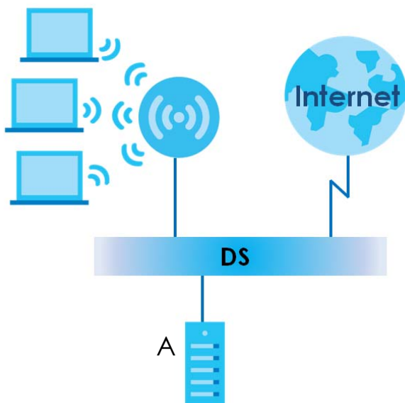
Figure 247 WPA(2) with RADIUS Application Example
