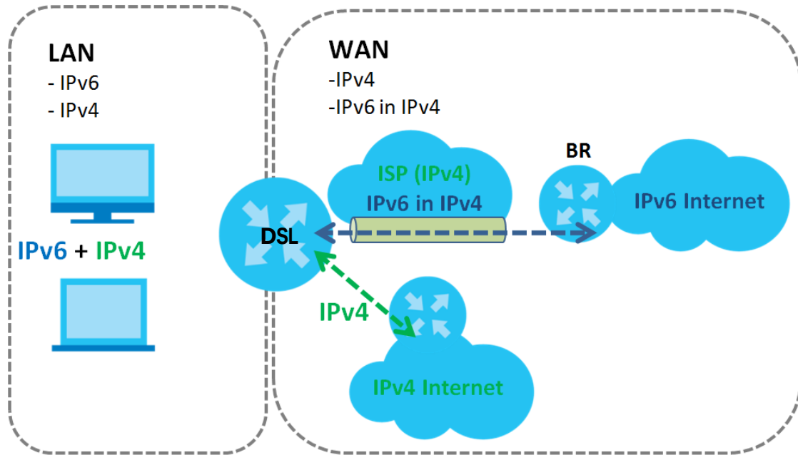
Figure 73 IPv6 Rapid Deployment
