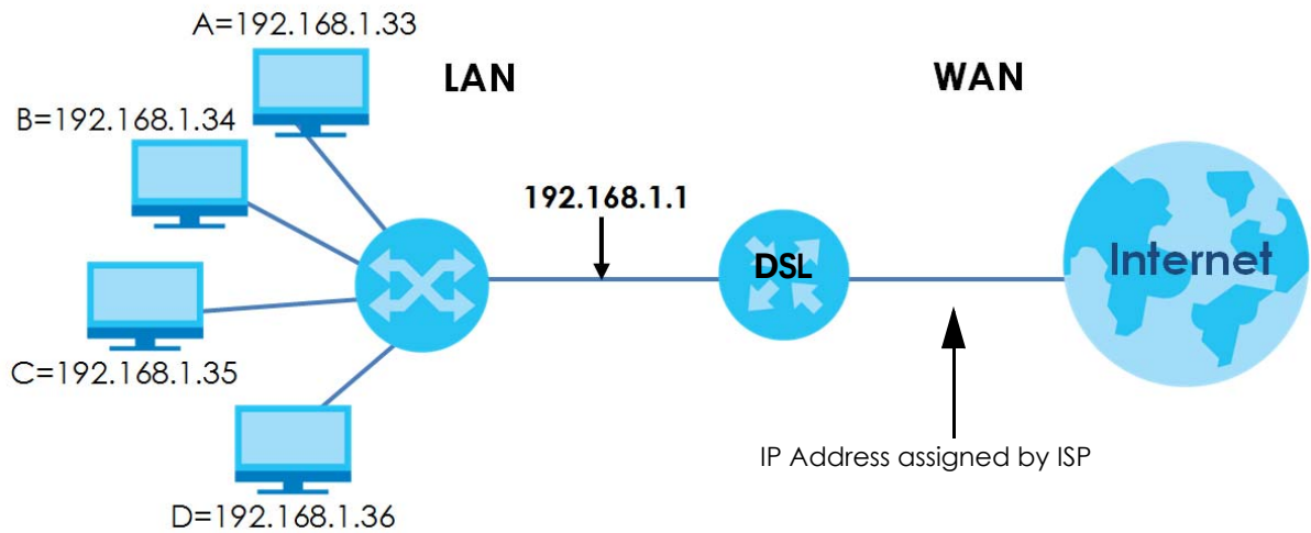
Figure 133 Multiple Servers Behind NAT Example
