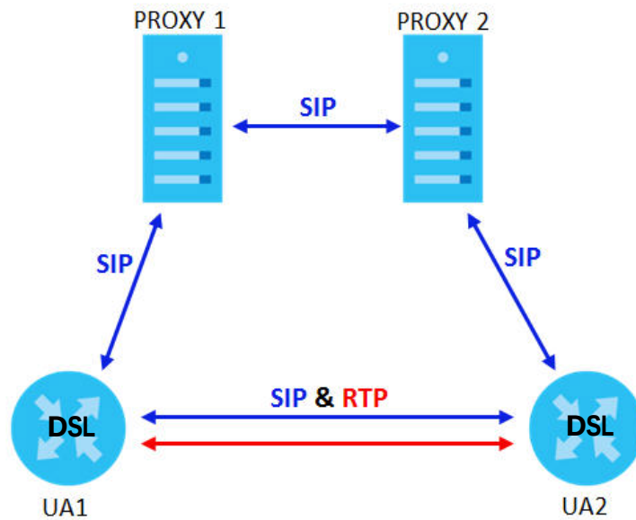
Figure 201 SIP Call Through Proxy Servers
