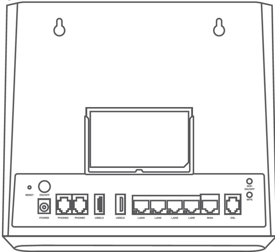
Figure 35 VMG8825-T50 Rear Panel
