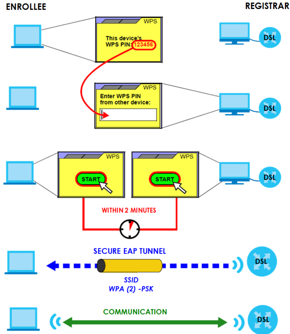
Figure 102 Example WPS Process: PIN Method
