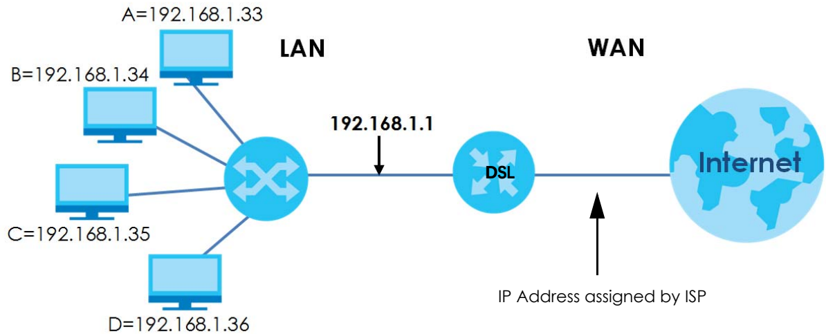
Figure 146 Multiple Servers Behind NAT Example
