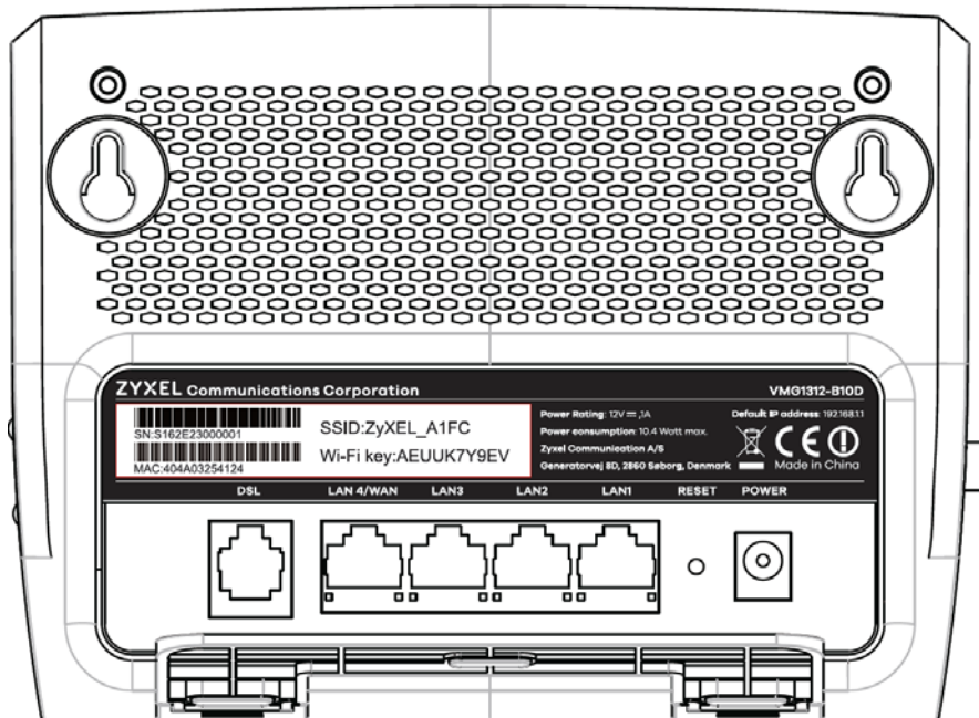
Figure 24 VMG1312-B10D Rear Panel
